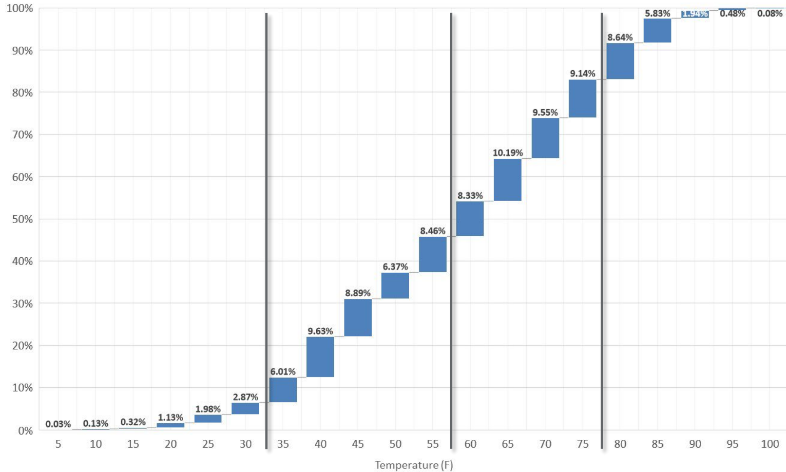
2010-2020 NYC Temperature
